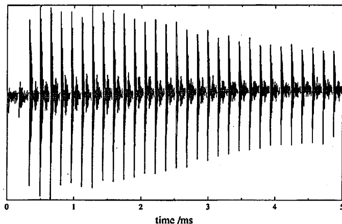
Fig. 2. The averaged 10000 point oscilloscope record obtained by adding wave forms from 100 pulses of Ar gas seeded with \text{CH}_2\text{Cl}_2 . On transition of the molecular beam through the cavity 32 consecutive microwave pulses were applied at excitation frequency of 9277.1203 MHz. The timings were chosen so that signal obtained for the first two microwave pulses illustrates spectrometer response just prior to the arrival of the gas pulse. Spurious transients from the first 15 \mu\text{s} directly following the 200 ns exciting microwave pulse were suppressed for clarity and intensities are in arbitrary units.
