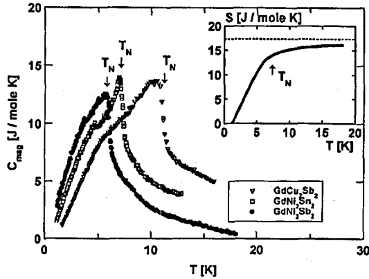
Fig. 2. Magnetic contribution to the specific heat. Inset: magnetic entropy of \text{GdNi}_2\text{Sb}_2 ; the dashed line indicates the R \ln 8 limit.
