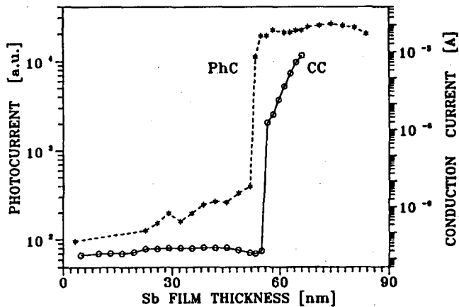
Fig. 2. The dependence of the conduction current and integral photoemission current on the Sb layer thickness.
