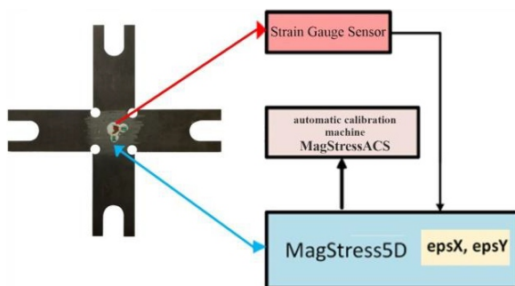
Fig. 3. Measuring system operation scheme.
