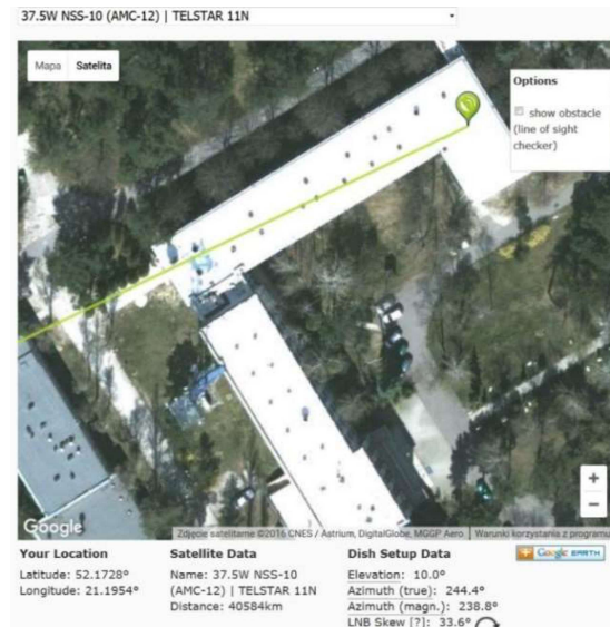
Fig. 3. Direction of satellite dish for TWSTFT in NIT's location for the T11N satellite (see [10]).
