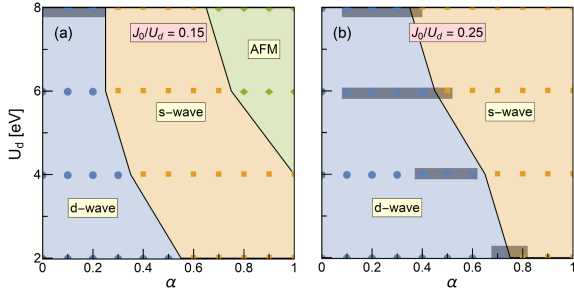
Fig. 5. Phase diagram in (U_d, \alpha) plane for increasing Hund's exchange, i.e., increasing ratio J_0/U_d : (a) J_0/U_d = 0.15 , and (b) J_0/U_d = 0.25 . Antiferromagnetism (AFM) is found only in (a) for J_0/U_d = 0.15 and U_d > 4 eV. The pairing has s - and d -wave symmetry, depending on the parameters. Tendency towards triplet pairing is highlighted by gray boxes; the points mark the parameters, at which the calculations were performed.
