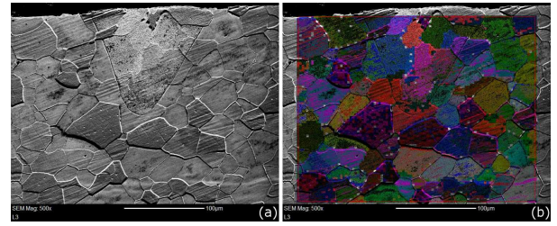
Fig. 5. Cross-sectional microstructures in vicinity of fiber laser induced HAZ regions in M540-50A visualized by: (a) conventional SEM imaging, (b) EBSD-IPF mapping (50 W, 20 µs).
