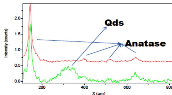
Fig. 5. Raman spectra of the investigated samples, red line (top) \text{TiO}_2 , green line (bottom) \text{TiO}_2 with quantum dots layer on the top.
