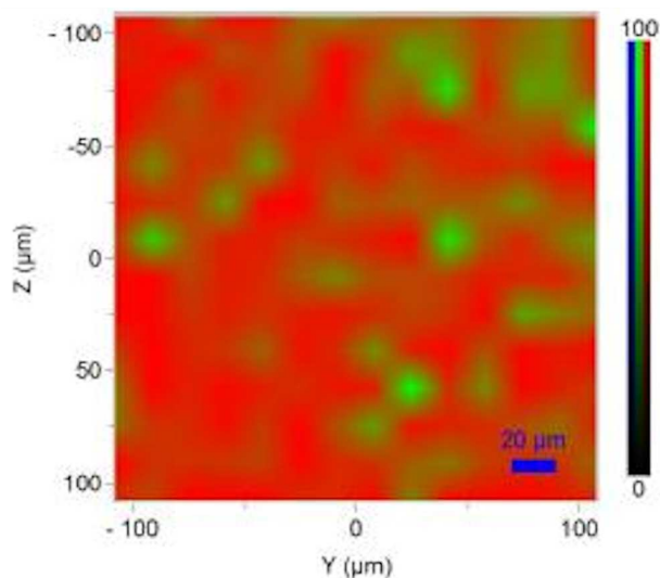
Fig. 3. The surface map of the \text{TiO}_2 photoanode is made using the Raman spectroscopy.
