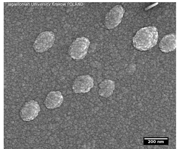
Fig. 2. High magnification SEM image of \text{TiO}_2 surface made using PVD technique.
