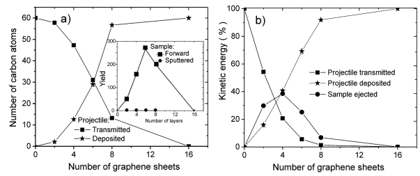
Fig. 2. Dependence of (a) the number of transmitted and sample-deposited projectile atoms and (b) the percentage of the primary kinetic energy carried by the transmitted projectile atoms, ejected sample atoms, as well as the energy deposited in the sample (projectile deposited) on the number of graphene sheets for 10 keV C_{60} projectiles at normal incidence. Inset to part (a) shows dependence of a number of sample atoms ejected in the forward and sputtered directions on the sample thickness.
