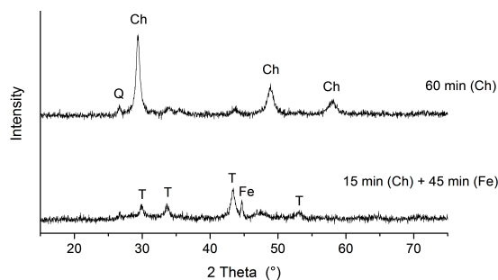
Fig. 3. X-ray diffraction patterns for \text{CuFeS}_2 (Slovinky) milled for 60 min (top) and mixture of the \text{CuFeS}_2 with Fe milled for 60 min (bottom): for 15 min, pure chalcopyrite was milled and then Fe was added and the mixture was then milled for further 45 min; Ch — \text{CuFeS}_2 , T — FeS.
