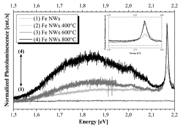
Fig. 3. Photoluminescence spectra registered for (1) as-prepared Fe NWs; (2) Fe NWs annealed at 400 °C; (3) Fe NWs annealed at 600 °C and (4) Fe NWs annealed at 800 °C. Inset: more detailed view on the PL spectra in the range from 2.1 eV to 2.2 eV. All spectra recorded for laser excitation of 532 nm.
