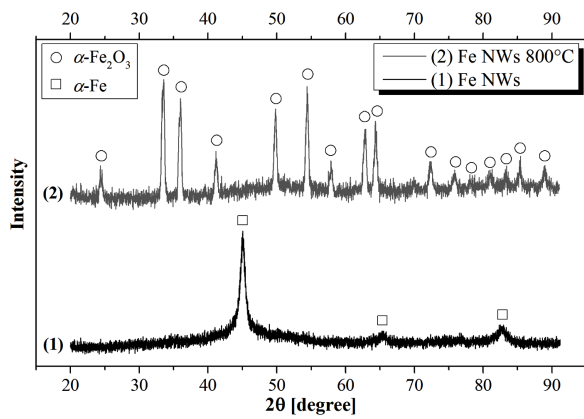
Fig. 1. XRD patterns of (1) as-prepared iron nanowires and (2) iron nanowires annealed at 800 °C. Positions of peaks determined according to JCPDS cards with numbers 87-0722 ( \alpha -Fe) and 84-0311 ( \alpha - \text{Fe}_2\text{O}_3 ).
