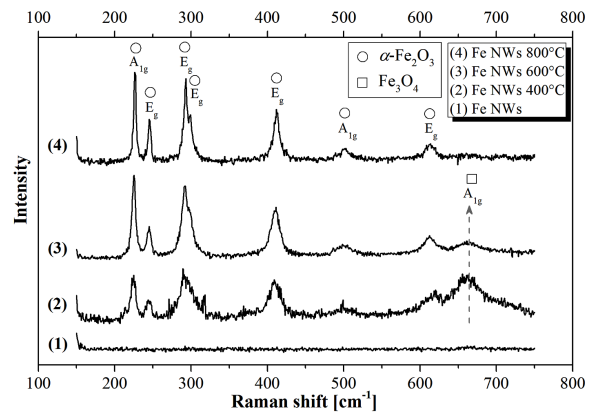
Fig. 2. Raman spectra of (1) as-prepared iron nanowires and Fe NWs annealed at (2) 400 °C, (3) 600 °C, and (4) 800 °C.
