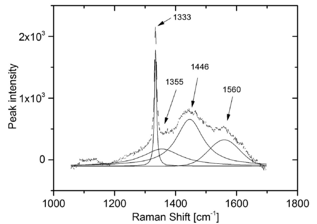
Fig. 3. Example deconvolution of Raman spectra in the range of 1000 – 1800\ \text{cm}^{-1} , four main peaks were marked. The 120 min deposition using DMSO-based colloid seeding is presented.
