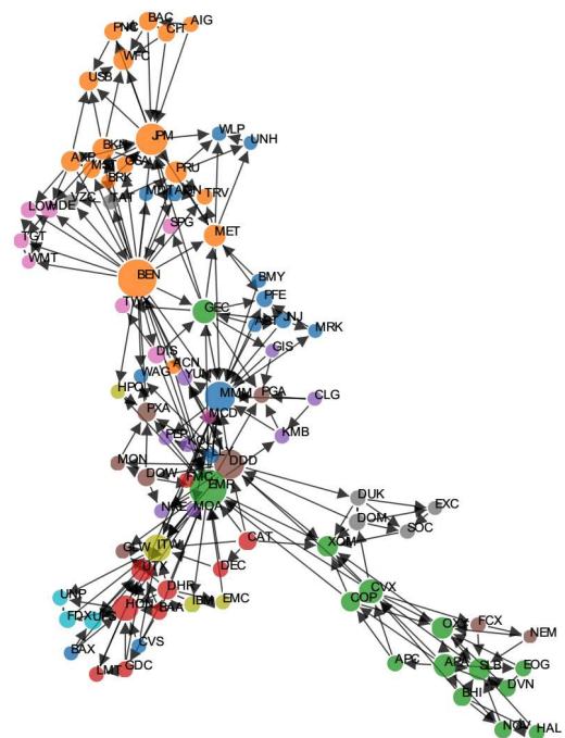
Fig. 4. Partial mutual information planar graph.
