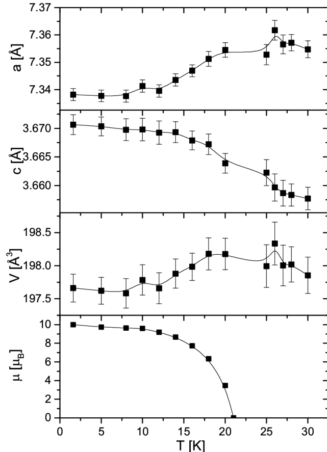
Fig. 2. Temperature dependence of the values of the lattice parameters a and c , unit cell volume V and the Tb magnetic moments for \text{Tb}_2\text{Ni}_{1.78}\text{In} compound.
