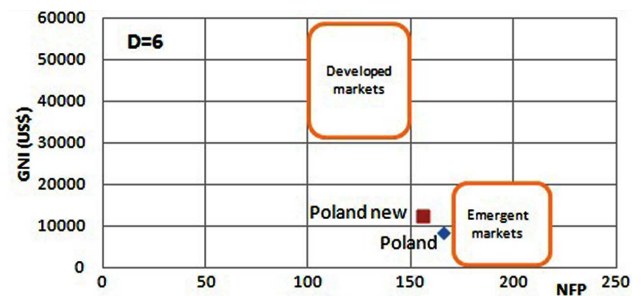
Fig. 1. The gross national income (GNI) per capita as a function of NFP with D = 6 .
