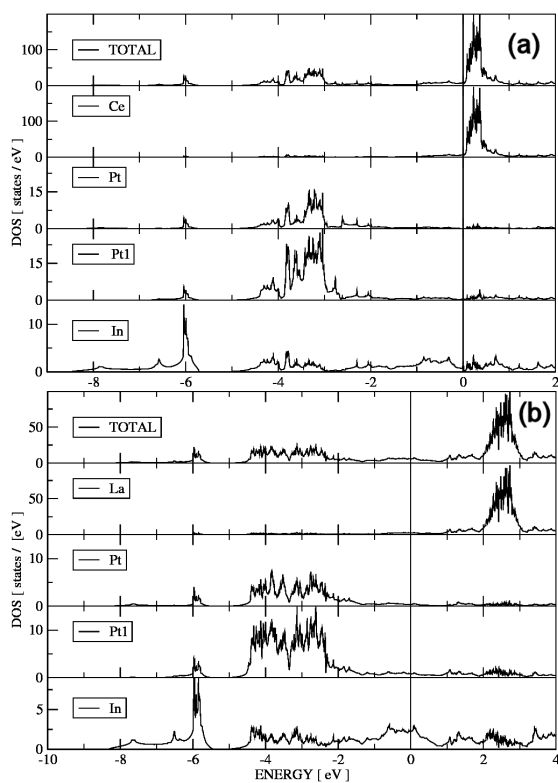
Fig. 2. Total density of states and the contribution from Ce or La, Pt and In to the total density of states for CePtIn (a) and LaPtIn (b) calculated in the scalar-relativistic approximation.
