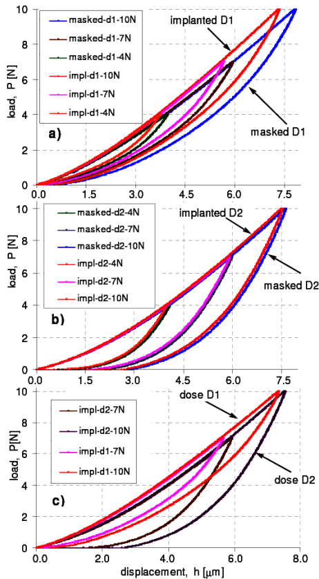
Fig. 2. Microindentation (a spherical tipped indenter R = 200 \mu\text{m} ) P – h curves for masked and ion implanted areas: with D1 = 1 \times 10^{17} \text{ cm}^{-2} (a); with D2 = 4 \times 10^{18} \text{ cm}^{-2} (b); for ion implanted with fluences D1 and D2 areas of NiTi samples (c).
