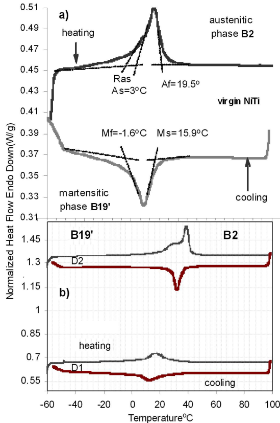
Fig. 1. Phase transformation temperatures obtained by DSC test for virgin NiTi SMA (a) and for N^+ implanted ( D1 = 1 \times 10^{17} \text{ cm}^{-2} , D2 = 4 \times 10^{18} \text{ cm}^{-2} ) NiTi alloy.
