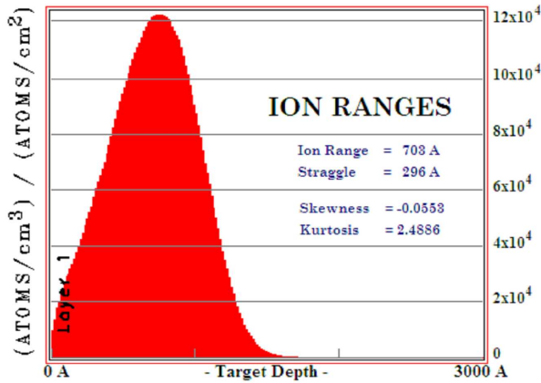
Fig. 5. SRIM-code prediction of 55 keV nitrogen ion range distribution in NiTi target.
