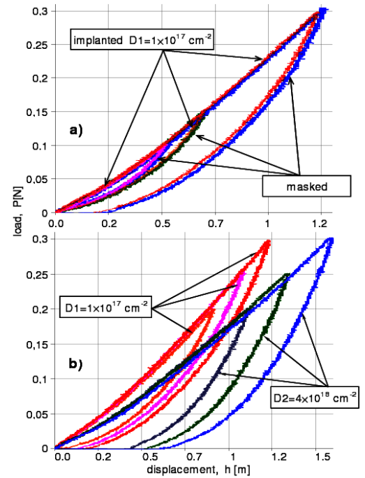
Fig. 3. Load–displacement curves received using a spherical tipped indenter R = 20 \mu\text{m} for masked and implanted ( D1 ) areas (a); for implanted NiTi surface at several D1 = 1 \times 10^{17} \text{ cm}^{-2} and D2 = 4 \times 10^{18} \text{ cm}^{-2} doses (b).
