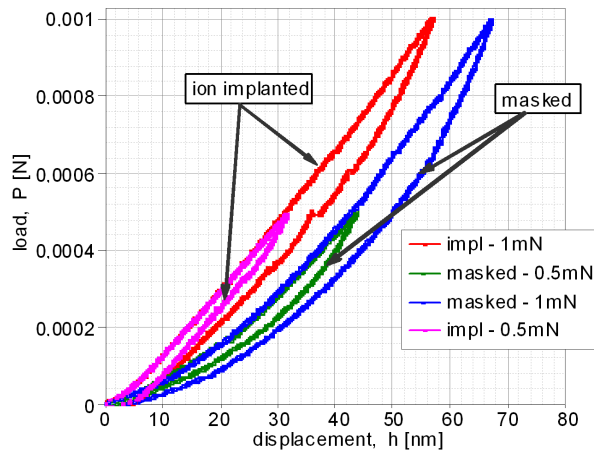
Fig. 4. Nanoindentation (spherical tipped indenter R = 2 \mu\text{m} ) P - h curves for masked and ion irradiated areas of NiTi sample, which was \text{N}^+ implanted with D1 = 1 \times 10^{17} \text{ cm}^{-2} .
