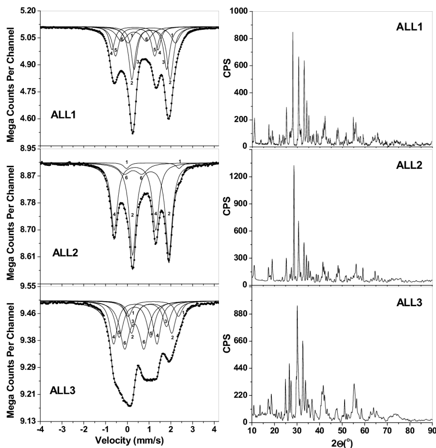
Fig. 1. (left hand plots) ^{57}\text{Fe} Mössbauer spectra at room temperature of allanite samples. Solid dots — experimental data; thick solid line — fitted curve; thin solid line — fitted doublets. (right hand plots) Corresponding XRD patterns.
