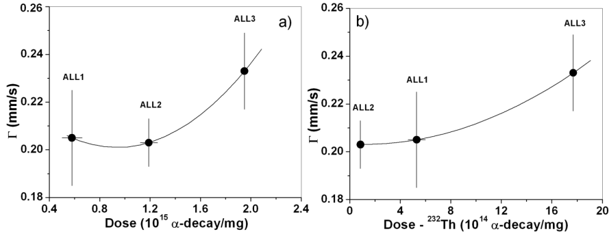
Fig. 5. Average line widths of \text{Fe}^{3+} components versus: (a) absorbed total \alpha -dose and (b) absorbed \alpha -dose from the ^{232}\text{Th} series. The solid lines represent polynomial regressions: \Gamma = 0.228 - 0.058D + 0.031D^2 and \Gamma = 0.203 - 0.0002D_{\text{Th}} + 0.0001D_{\text{Th}}^2 . The correlation coefficients are r = 0.87 and 0.98 , respectively.
