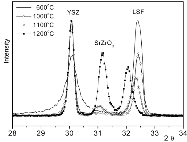
Fig. 3. XRD spectra of YSZ film on LSF perovskite (film sintered at various temperatures).
