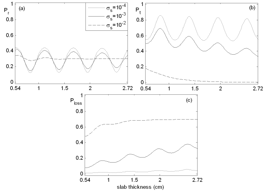
Fig. 4. The reflected (a), the transmitted (b), and the loss power (c) for TE wave against the slab thickness.
