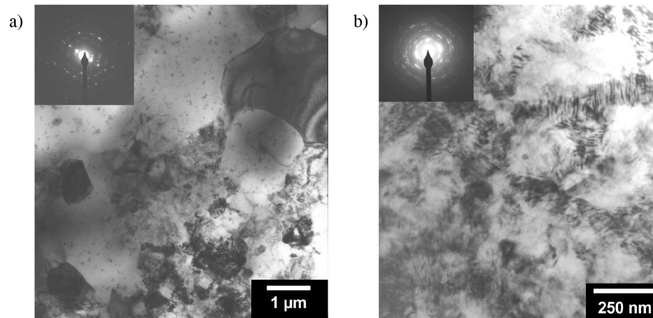
Fig. 2. Bright-field TEM image of (a) Mg and (b) Mg-10%Gd alloy deformed by HPT.
