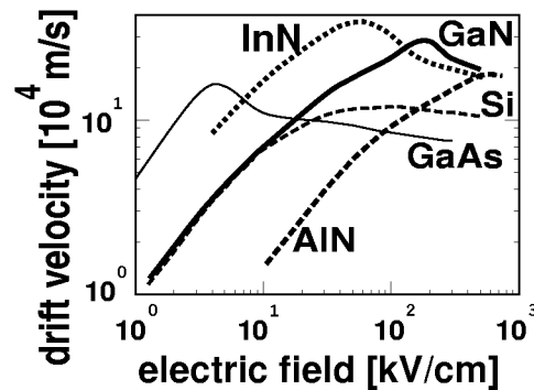
Fig. 5. Calculated electron drift velocities of GaN, AlN, and InN in comparison with GaAs and Si.
