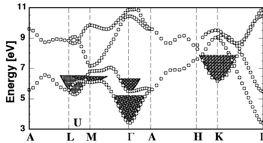
Fig. 2. Conduction bands of wurtzite GaN as obtained from density functional calculations.
