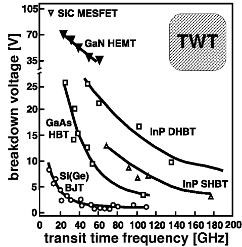
Fig. 1. Breakdown voltage and transit time frequency of electron devices based on various materials. The region covered by travelling wave tubes (TWT) is also marked.
