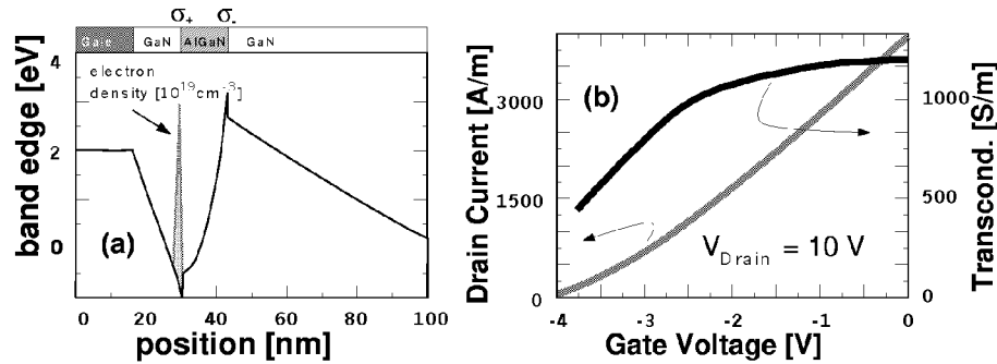
Fig. 9. Monte Carlo results for a 300 nm gate length inverted GaN/ \text{Al}_{0.40}\text{Ga}_{0.60}\text{N} HFET. (a) Self-consistent band edge profile for -1 \text{ V} gate voltage and 10 \text{ V} drain voltage. The channel electron density is indicated schematically. (b) Drain current and transconductance versus gate voltage at 10 \text{ V} drain voltage.
