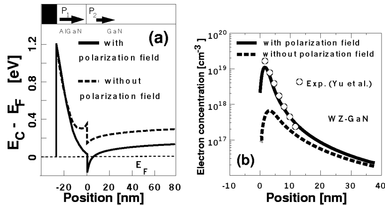
Fig. 4. Calculated results for a Al 0.15 Ga 0.85 N/GaN heterostructure with (full lines) and without (dashed lines) spontaneous and piezoelectric fields. A homogeneous n -doping background of 10^{16} \text{ cm}^{-3} throughout the structure has been assumed. (a) Self-consistently computed conduction band edge profile along the growth direction. (b) Calculated electron density in comparison with published experimental values.
