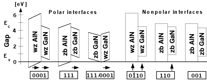
Fig. 3. Predicted band lineups for several AlN/GaN interfaces. The growth direction is given in boxes beneath each interface. The arrows indicate the direction of the spontaneous or strain-induced piezoelectric polarization. Polar interfaces possess an interface charge. The corresponding electric field induces a band bending which is indicated schematically.
