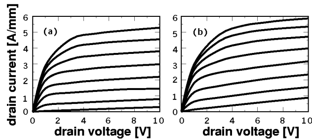
Fig. 6. Drain current characteristics for gate lengths (a) 300 nm and (b) 150 nm, as obtained from Monte Carlo simulations for \text{Al}_{0.30}\text{Ga}_{0.70}\text{N}/\text{GaN} HFET. The various gate voltages are given in steps of 1 V and begin with -8.4 eV (the lowest line).
